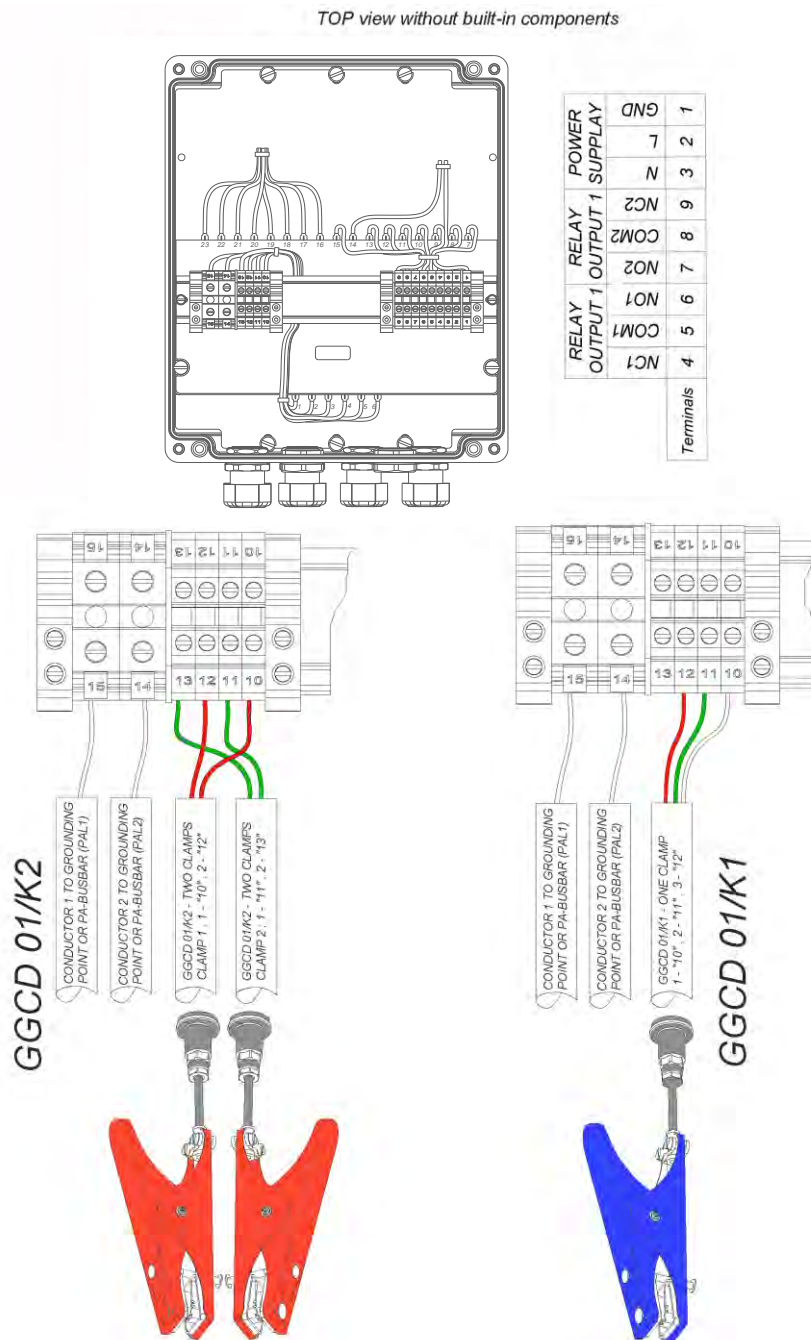
Electric connection scheme of cables and conductors:
