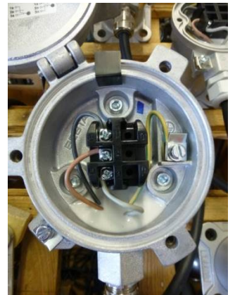
XU.. housing
