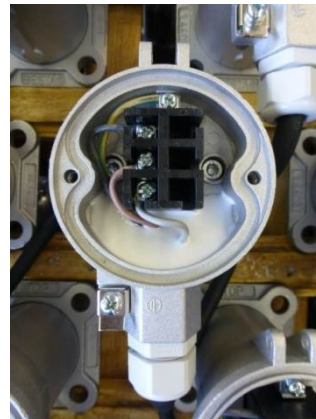
U.B.. and ZU.. housing
